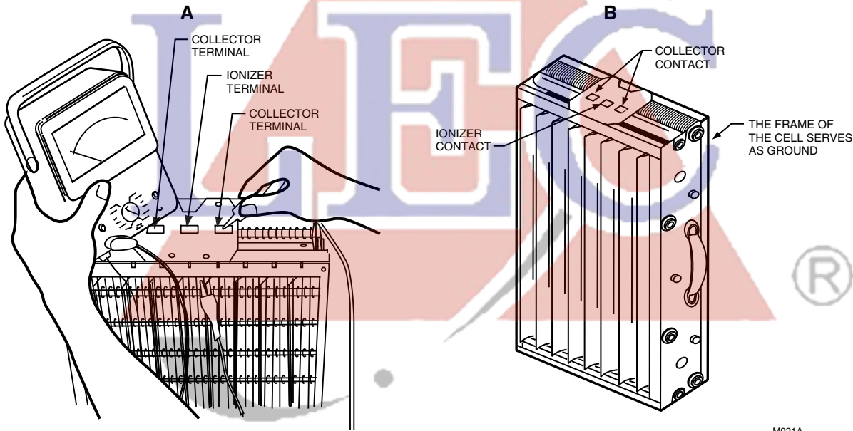
Fig. 20. Checking cells for short circuits.
