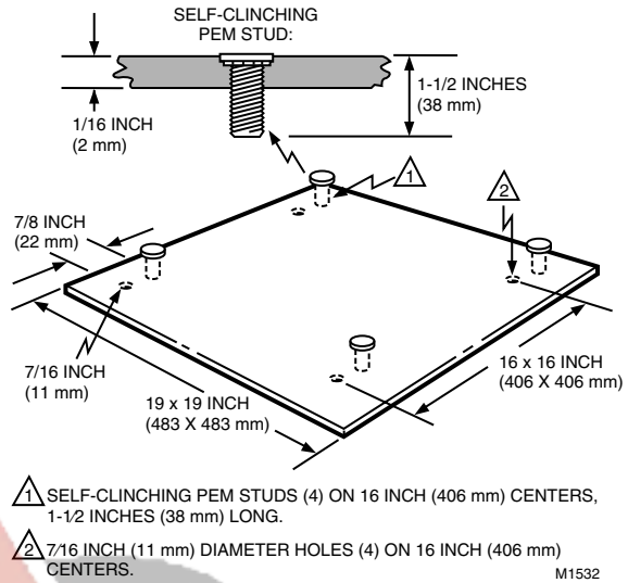
Fig. 10. Mounting F90 using 272577A Transition Plate.
