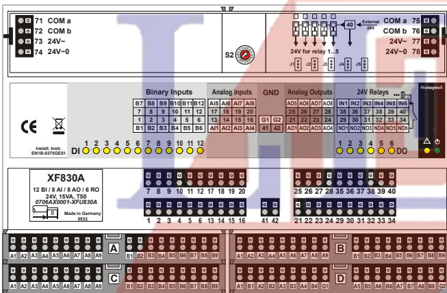
Fig. 22. XF830A mixed Excel 800 Panel Bus I/O module, shown with 4 optional aux. terminal blocks (top view)
