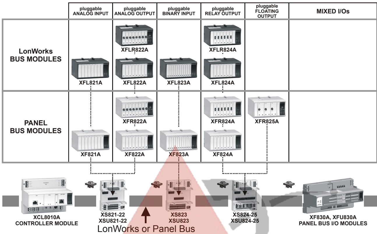
Fig. 2. Overview of Excel 800 Modules Table 1. Overview of Excel 800 Modules
