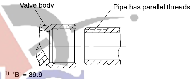
Fig. 24. 3/4" BSPP internal (Rp 3/4)
