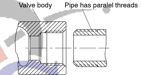
Fig. 16. 1/2" BSPP internal (Rp 1/2")
