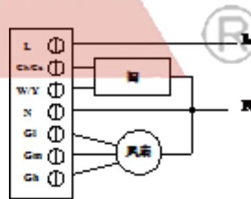
Typical wiring for ON/OFF control in 2 pipes Heat/Cool/1H1C (VC6013)
