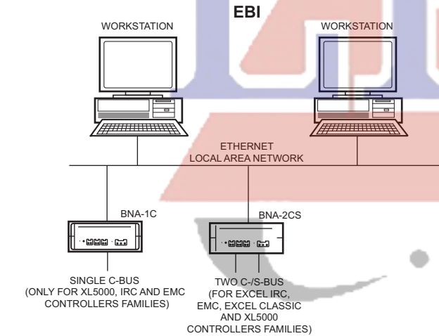
Fig. 1. Application block diagram.
